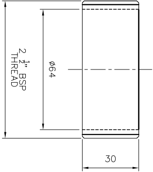
(SCALE:1:4) DETAIL-A BUSH FOR COUPLER
